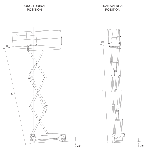
Stability for COMPACT 8 (COMPACT 2032E) - COMPACT 8 CU
